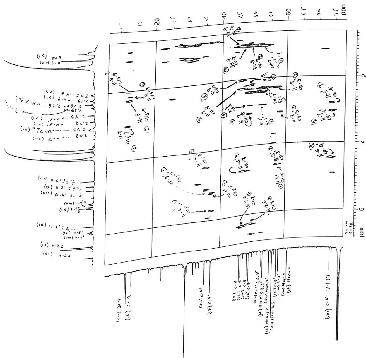
Figura 85 : Espectro de RMN 2D ^1\text{H} x ^{13}\text{C} HMQC, região 0,7-6,8 x 10,0-75,0 ppm das neolignanas VIII e IX (125 MHz, \text{CDCl}_3 )
