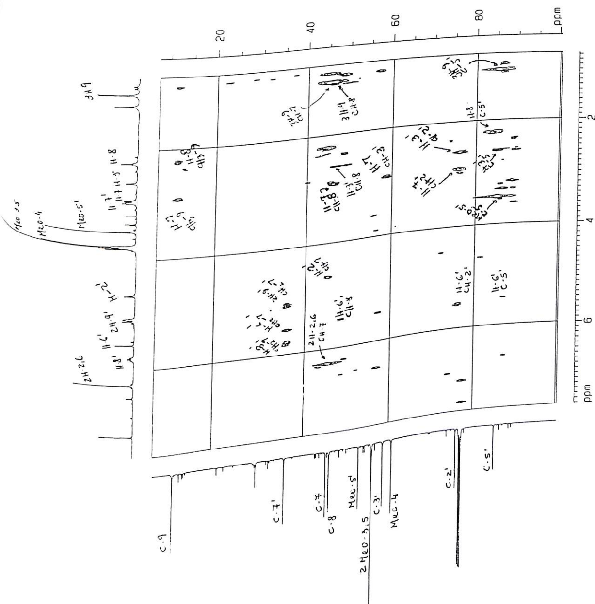
Figura 67 : Espectro de RMN 2D ^1\text{H} \times ^{13}\text{C} HMBN, região 1,0-8,0 x 10,0-100,0 ppm da neolignana VII (125 MHz, \text{CDCl}_3 )
