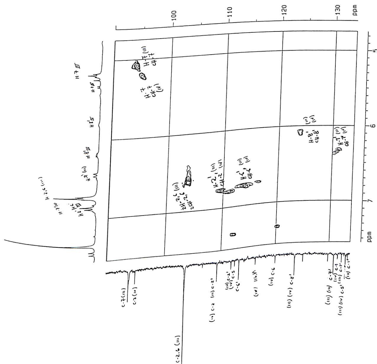
Figura 22 : Espectro de ^1\text{H} \times ^{13}\text{C} HMQC, região 4,7-7,5 x 90,0-135,0 das neolignan III e IV (125 MHz, \text{CDCl}_3 )
