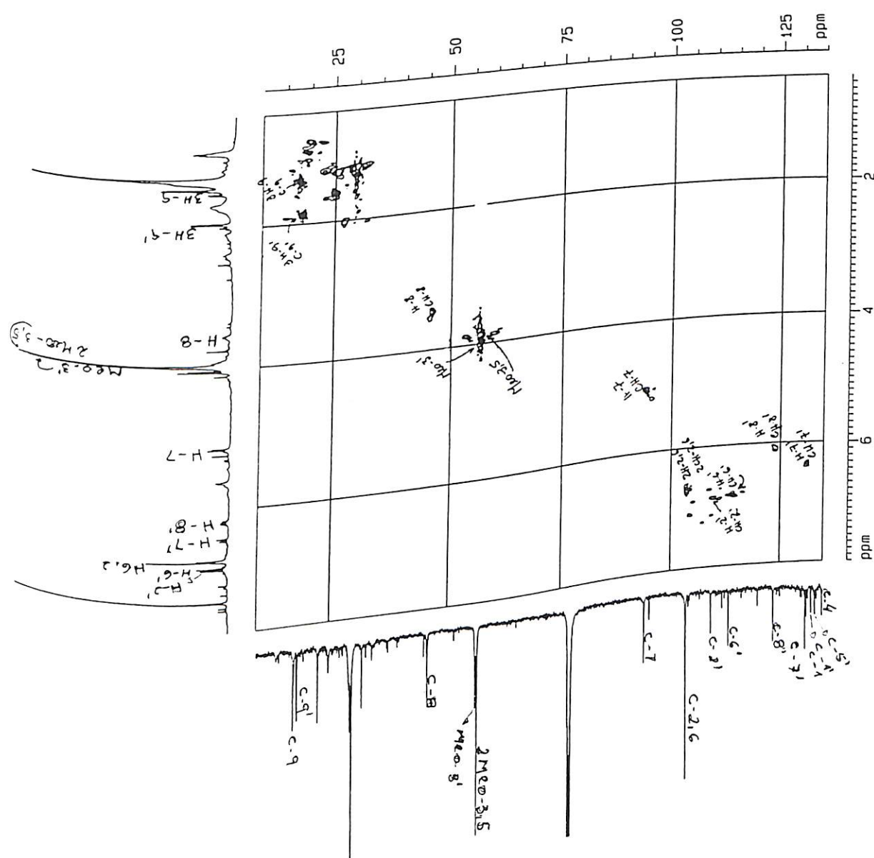
Figura 36 : Espectro de RMN 2D - ^1\text{H} \times ^{13}\text{C} HMQC, região 1,0-7,0 x 20,0-135,0 ppm da neolignana V (125 MHz, \text{CDCl}_3 )
