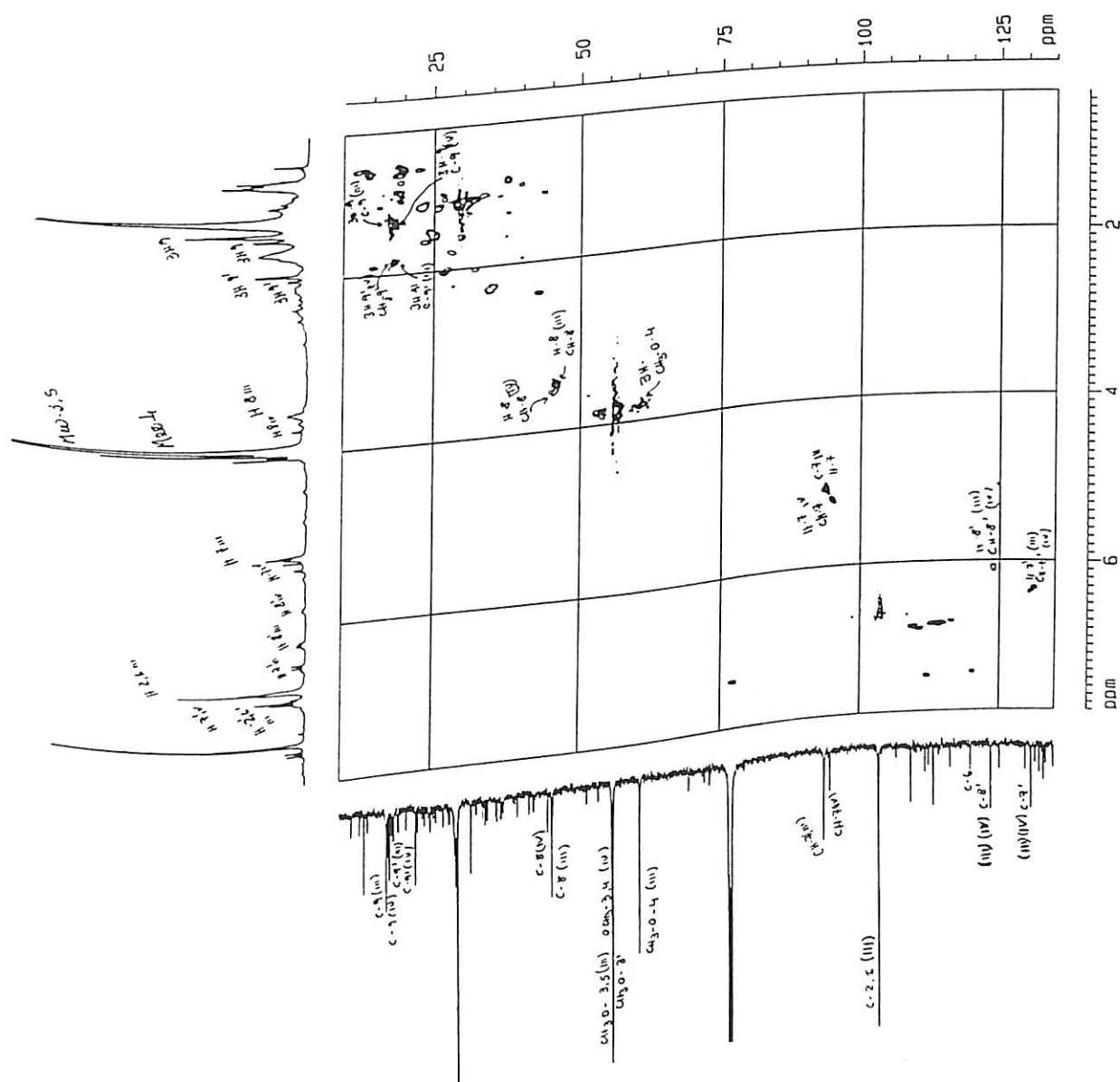
Figura 21 : Espectro de ^1\text{H} \times ^{13}\text{C} HMQC, região 0,0-7,0 x 0,0-130,0 das neolignanas III e IV (125 MHz, \text{CDCl}_3 )
