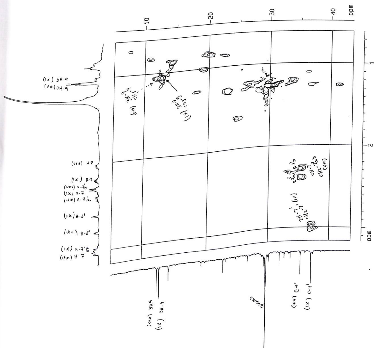
Figura 82 : Espectro de RMN 2D ^1\text{H} \times ^{13}\text{C} HMQC, região 1,6-3,0 x 5,0-45,0 ppm das neolignan VIII e IX (125 MHz, \text{CDCl}_3 )
