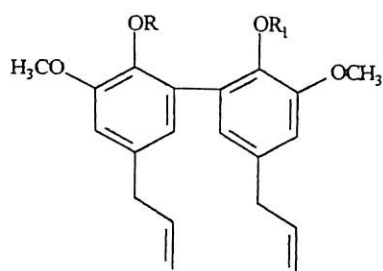
46 : R = R 1 = H
