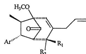
51 : R 1 = H, R 2 = OH - Macrophyllir
