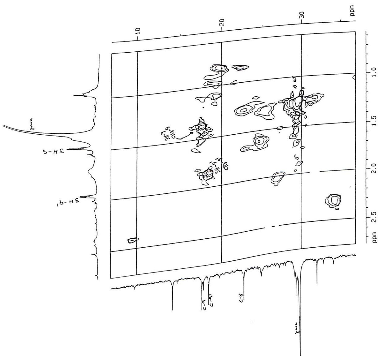
Figura 37 : Espectro de RMN 2D ^1\text{H} \times ^{13}\text{C} HMQC, região 0,5-2,7 x 10,0-36,0 ppm da neolignana V (125 MHz, \text{CDCl}_3 )
