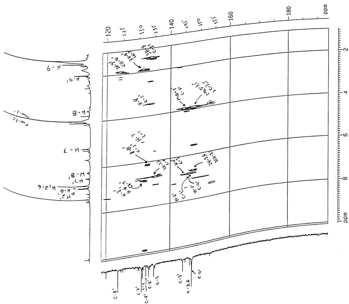
Figura 42 : Espectro de RMN 2D ^1\text{H} \times ^{13}\text{C} HMBN, região 1,5-10,0 x 120,0-195,0 ppm da neolignana V (125 MHz, \text{CDCl}_3 )
