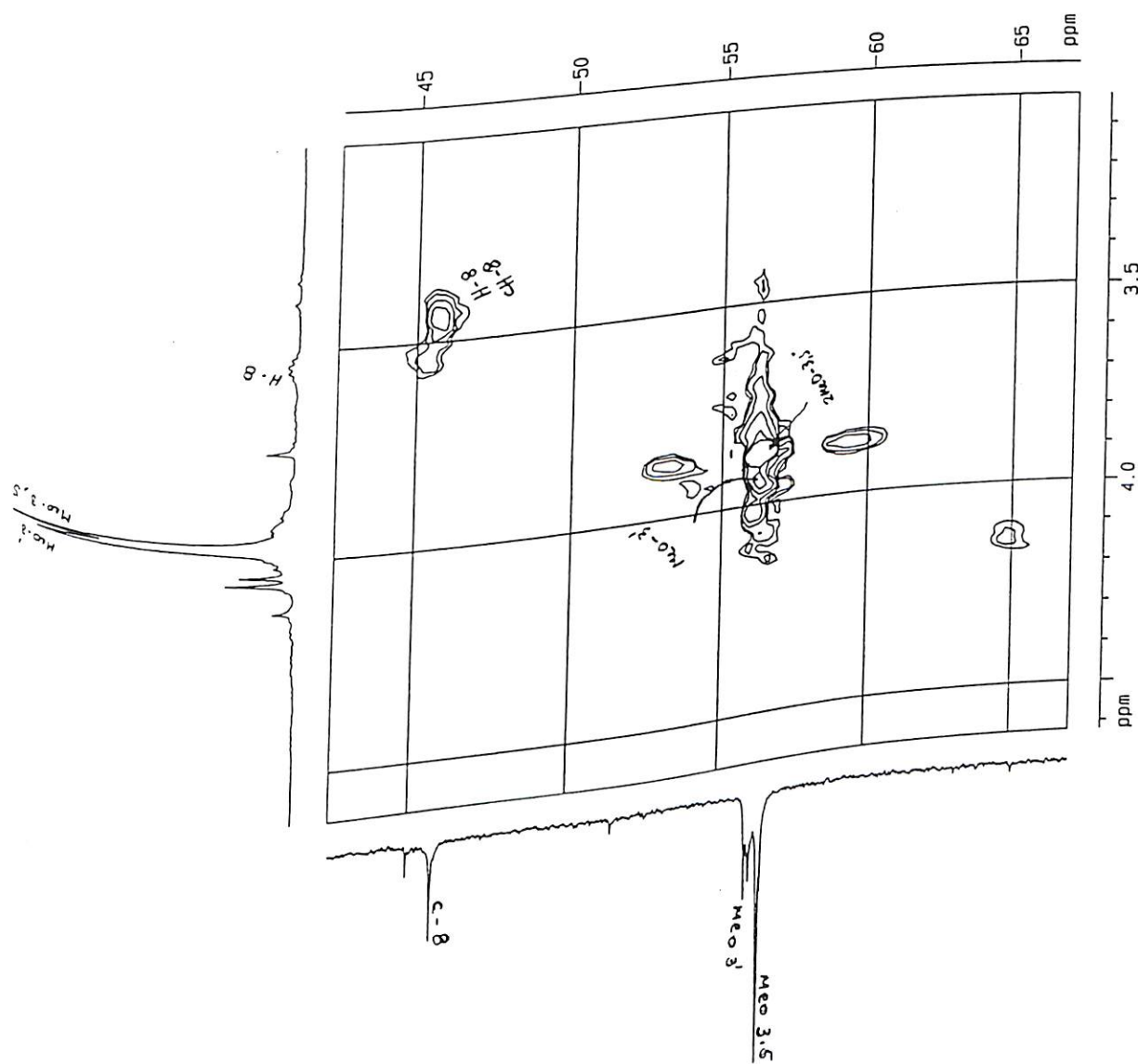
Figura 38 : Espectro de RMN 2D ^1\text{H} \times ^{13}\text{C} HMQC, região 3,0-4,6 x 40,0-70,0 ppm da neolignana V (125 MHz, \text{CDCl}_3 )
